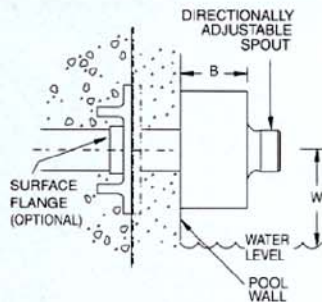
Surface Mounted Application
