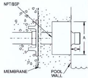
Flushwall Application
